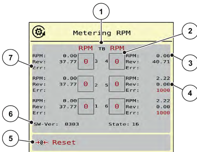
图 23: Test/diagnosis ; 示例: Metering RPM
