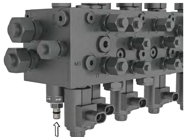
Abb. 16: Position LS/KS-Ventil
