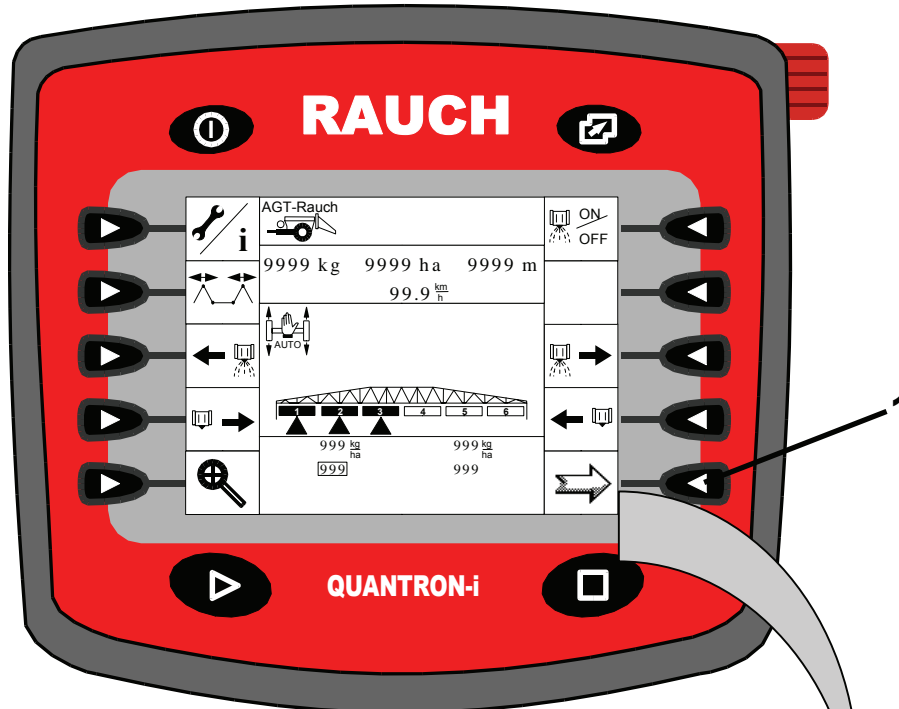
Operating screen 1
