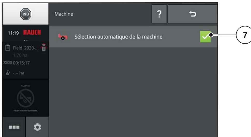
Figure 4.7 : Menu Machine
