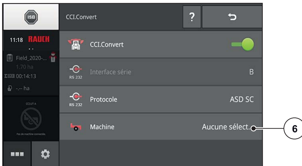
Figure 4.6 : Menu CCI.Config
