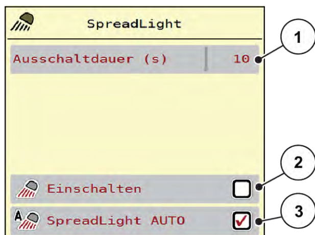
Abb. 25: Menü SpreadLight
